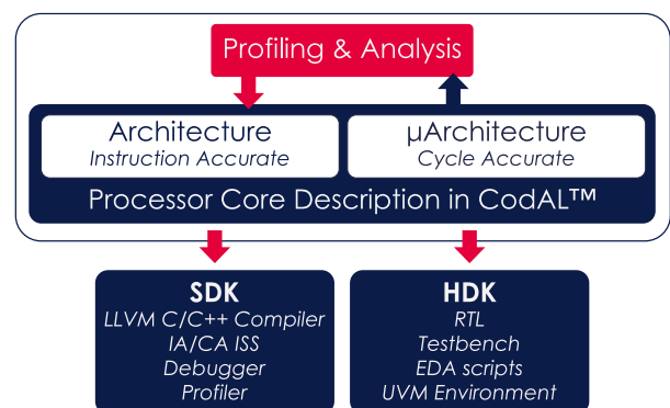
Cudasip Studio flow
